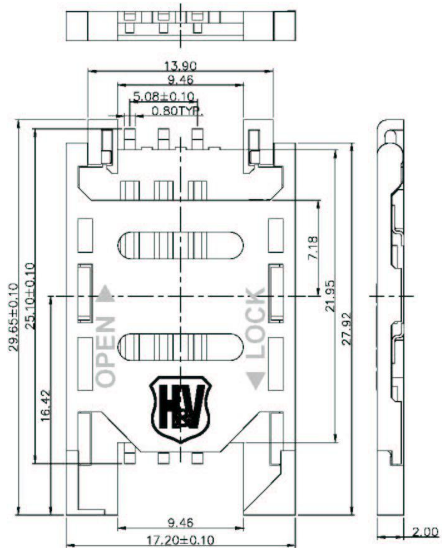
Unit: mm; Tolerances: ±0.15 mm Mechanical outline dimension
