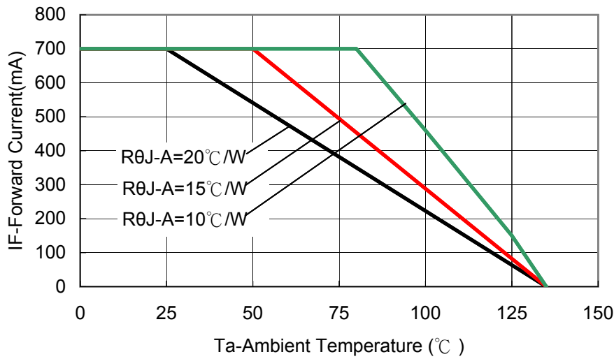
Fig 5a. Maximum Forward Current vs. Ambient Temperature. Derating based on TjMAX=135°C for White, Warm White, Blue and Green.
