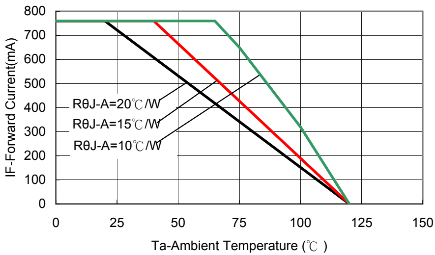
Fig 5b. Maximum Forward Current vs. Ambient Temperature. Derating based on TjMAX=120°C for Amber, Red-Orange and Red.
