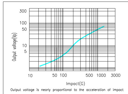
Output Voltage vs. Impact Response
